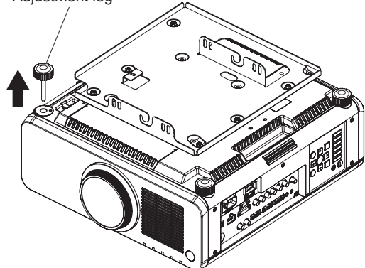
Adjustment leg
